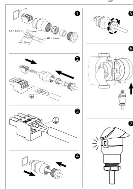
Electrical wiring
